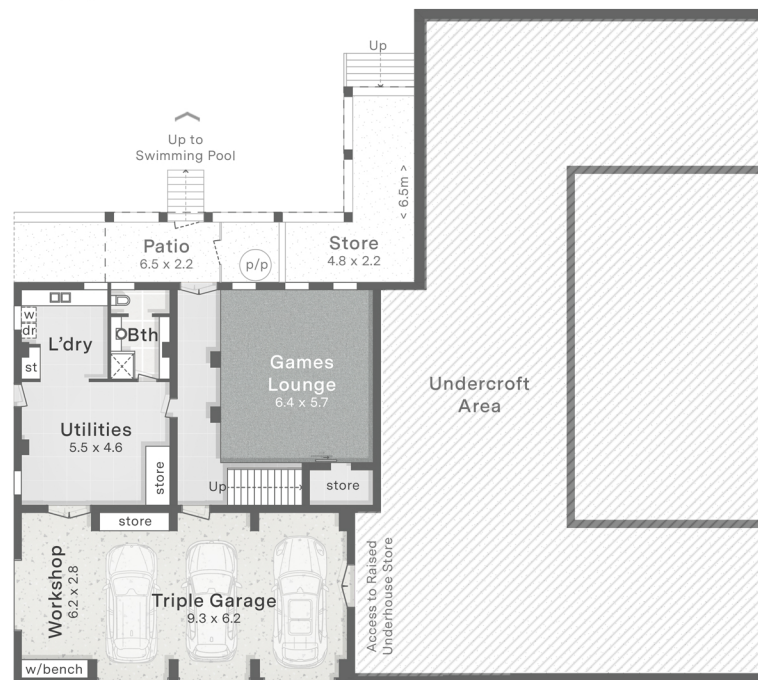
MAIN LEVEL Ceiling up to 5.6m
